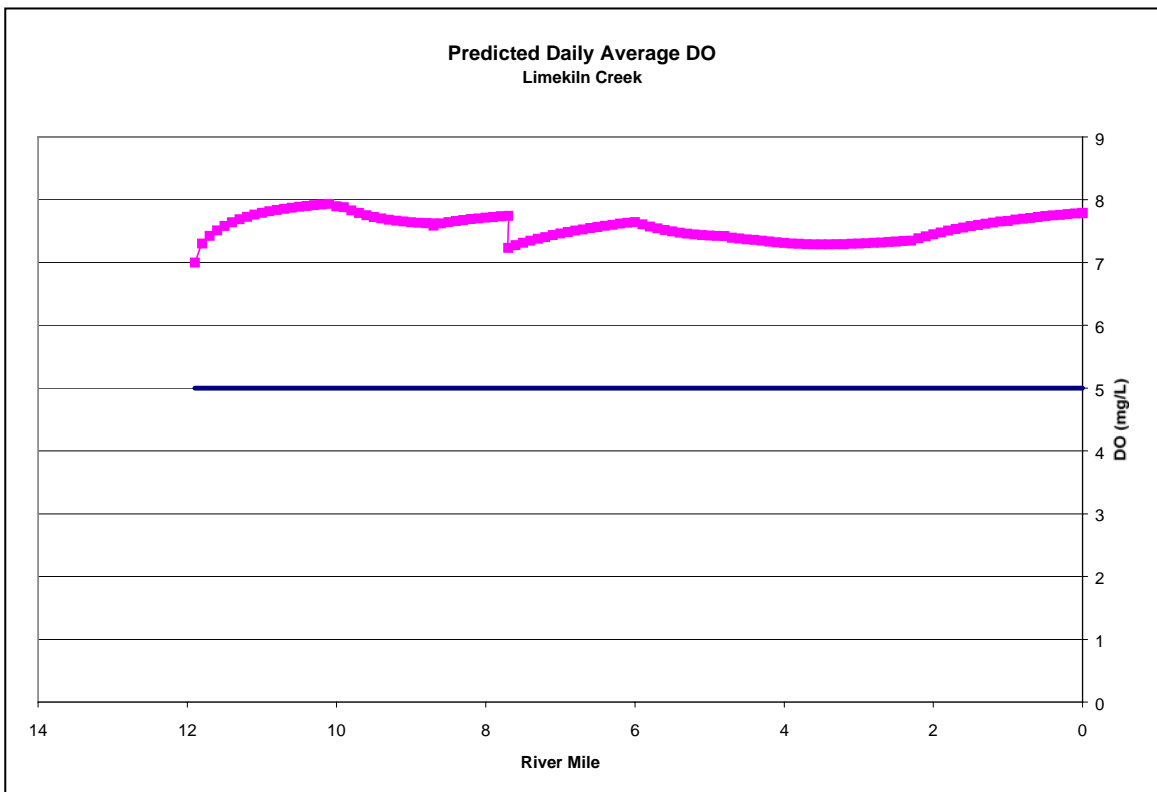
Figure 4.4. Baseline Model Output, Limekiln Creek
