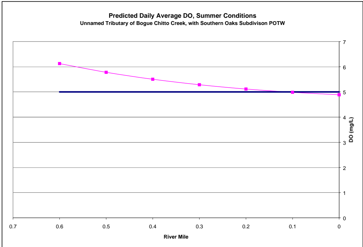
Figure 4.9. Load Reduction Scenario – Model Output, Unnamed Tributary
