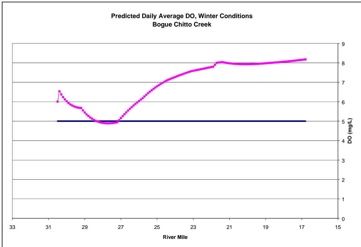
Figure 4.10. Load Reduction Scenario – Winter Model Output, Bogue Chitto Creek
