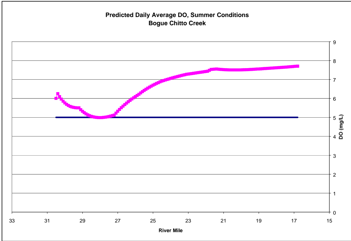
Figure 4.7. Load Reduction Scenario – Model Output, Bogue Chitto Creek
