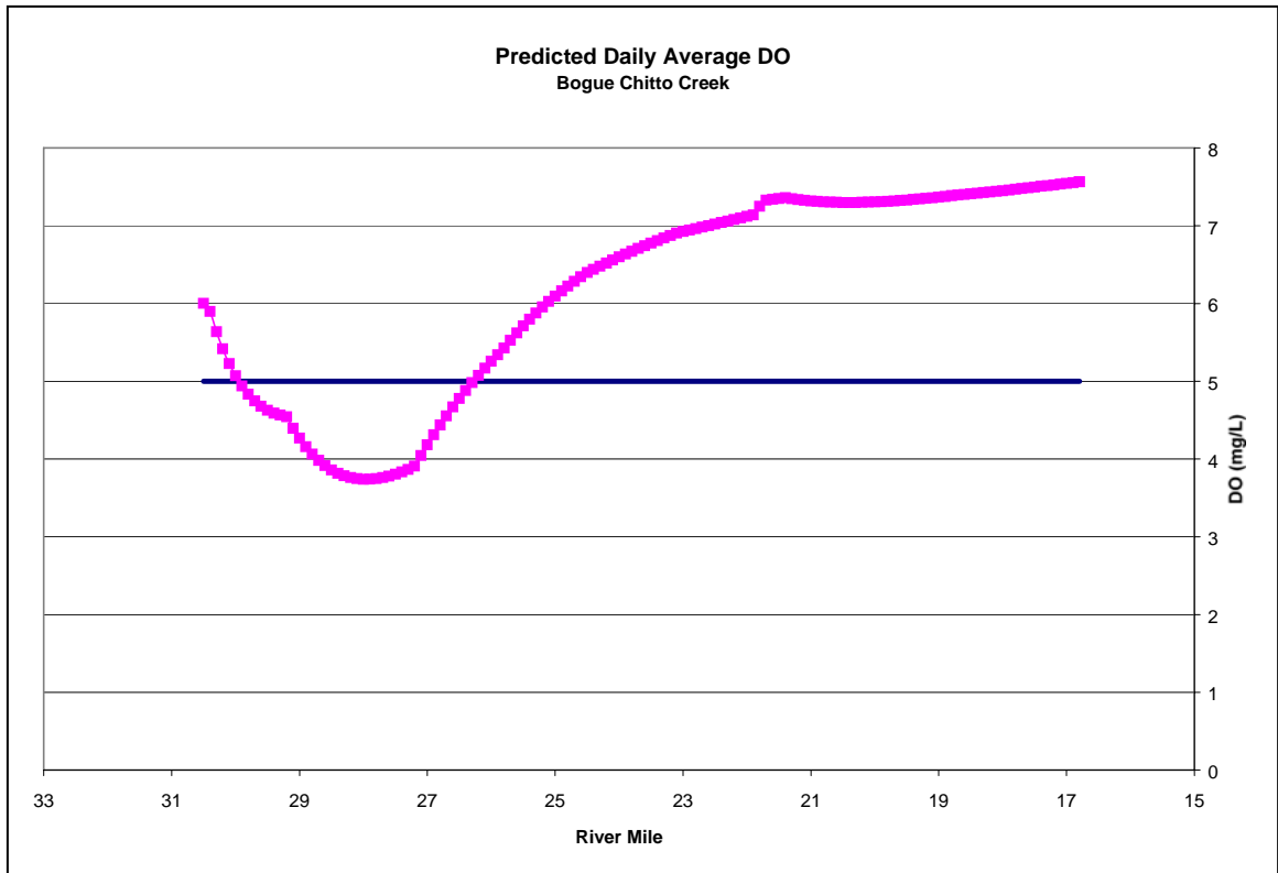
Figure 4.3. Baseline Model Output, Bogue Chitto Creek
