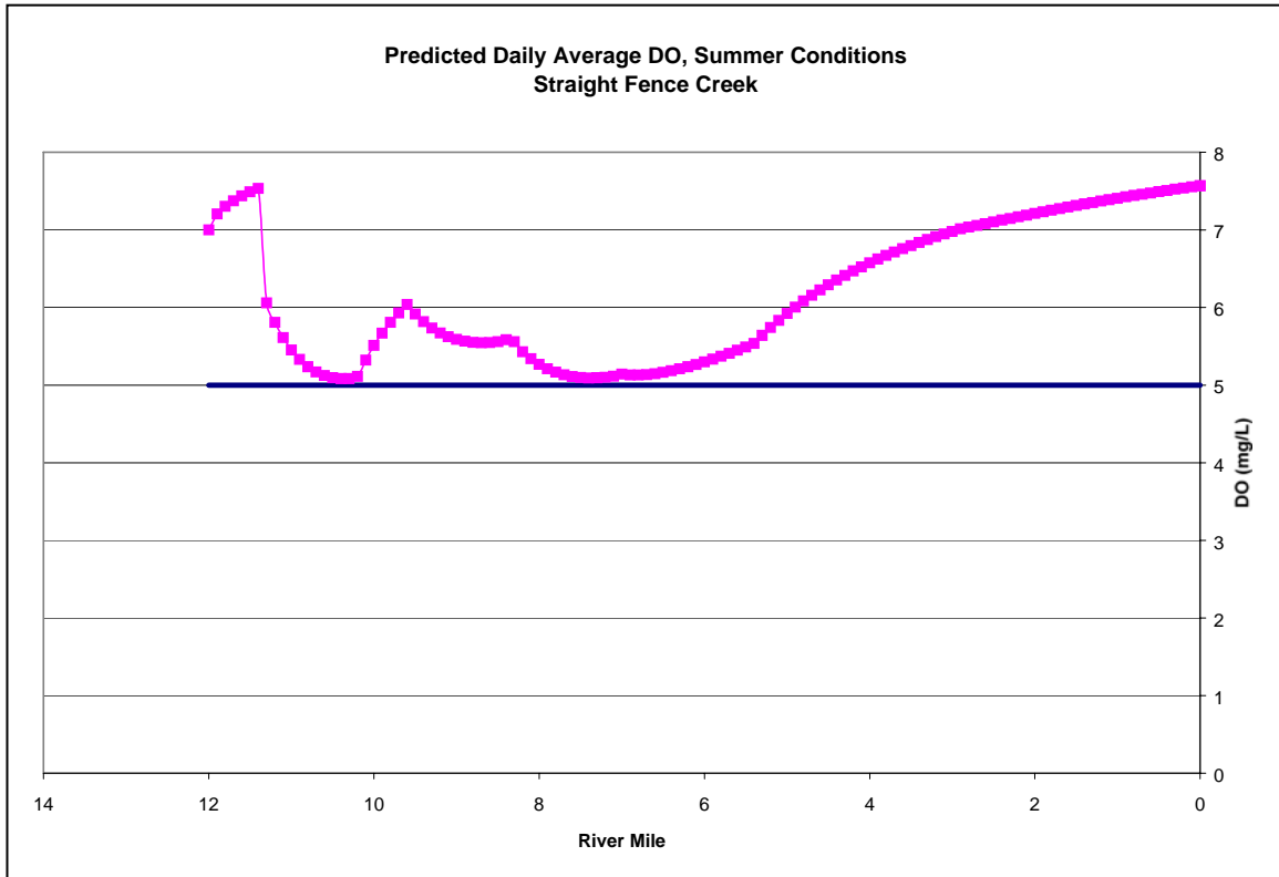
Figure 4.8. Load Reduction Scenario – Model Output, Straight Fence Creek
